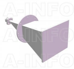
LB-62-25-C2-3.5FSPO Standard Gain Horn Antenna 12.4-18GHz 25dB Gain 3.5mm Female
